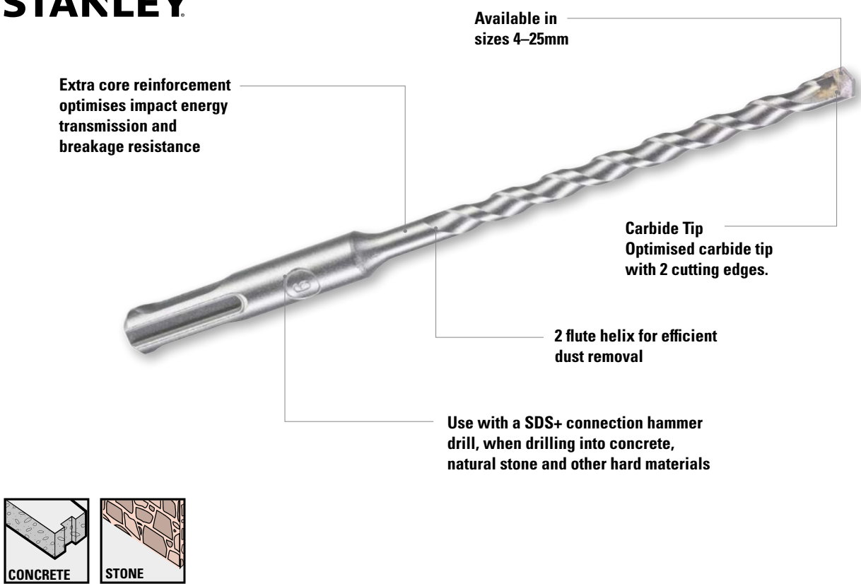
SDS+ CONNECTION - FOR HAMMER DRILLING INTO CONCRETE
