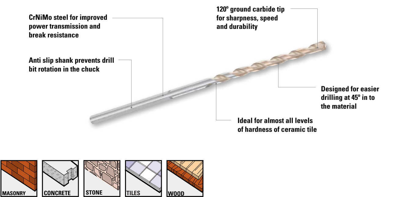
MULTI MATERIAL - FOR SIMULTANEOUS DRILLING IN MULTI-MATERIALS
